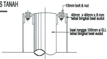
BUTIRAN B NOT TO SCALE
