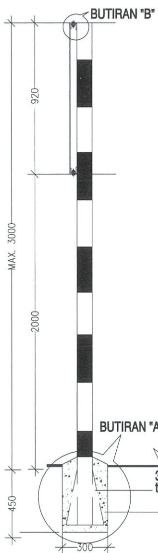
KERATAN A-A NOT TO SCALE
